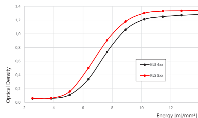
Dynamic sensitivity | KLS grades
