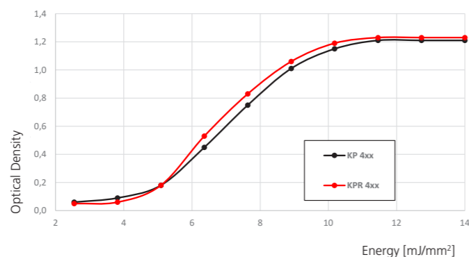
Dynamic sensitivity | KP/KPR grades
