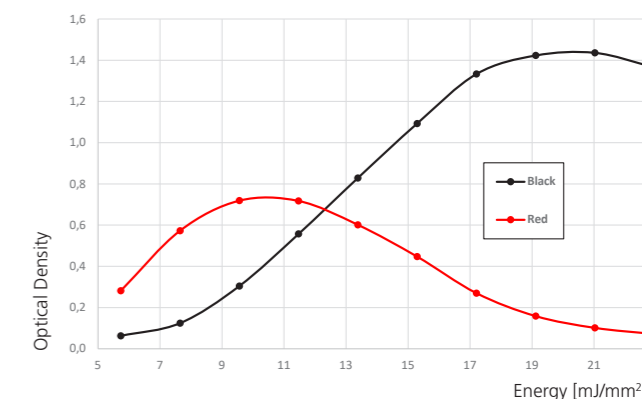
Dynamic sensitivity | KLRB 46B
